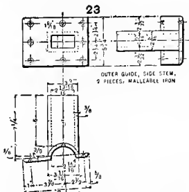
Figs. 1404-1406. Outer Side-stem Guide.
